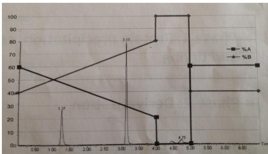
Figure 3.2. Linear gradient representation of mobile phases used during sample analysis. The column oven temperature was maintained at 45°C. This temperature provides a better separation in contrast to room temperature (Figure 3-3)
