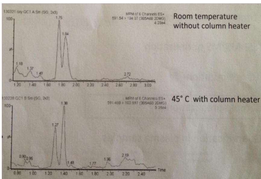
Figure 3.3. Separation of a plasma sample with and without a column heater.
