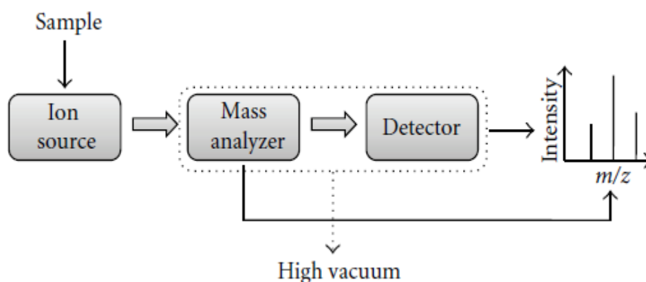
Figure 2.15. The basic components of mass spectrometer.
