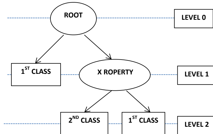
Figure 1. A generic decision tree for classification.
