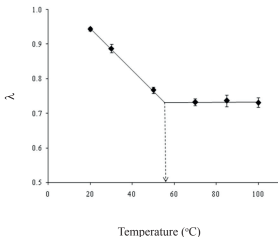
Fig. 4. Effect of temperature on the volumetric expansion coefficient ( \lambda ) of chickpea. Vertical bars on each data point indicate standard deviation.
