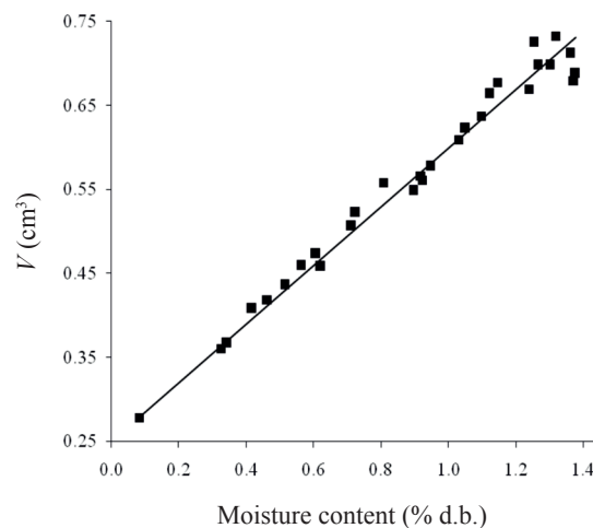
Fig. 2. Changes in the volume of chickpea seed during water absorption at 20°C.
