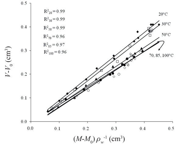
Fig. 3. Relationship between the volume of the water absorbed [(M-M_0) \rho_w^{-1}] and the volume increase in grains (V-V_0) during water absorption at different temperatures.
