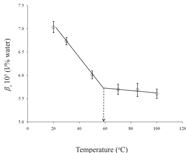
Fig. 5. Effect of temperature on the volumetric expansion coefficient ( \beta_v ) of chickpea. Explanations as in Fig. 4.
