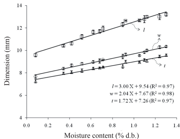
Fig. 1. Changes in the length ( l ), width ( w ) and thickness ( t ) of chickpea seed during water absorption at 20°C. Vertical bars on each data point indicate standard deviation.
