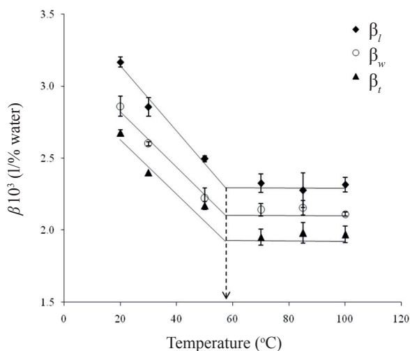
Fig. 6. Effect of temperature on the linear expansion coefficients ( \beta_l , \beta_w , \beta_t ) of chickpea. Explanations as in Fig. 4.
