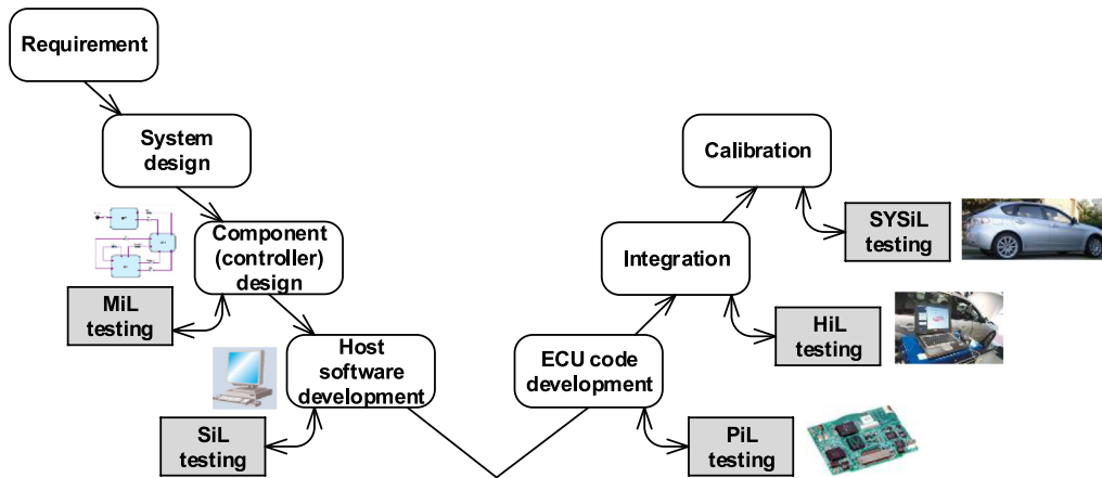
Fig. 12. The “V” development process including the X-in-the-loop testing phases (adapted from Day [72]).
