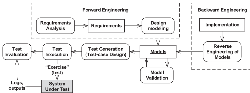
Fig. 11. General process of model-based testing.
