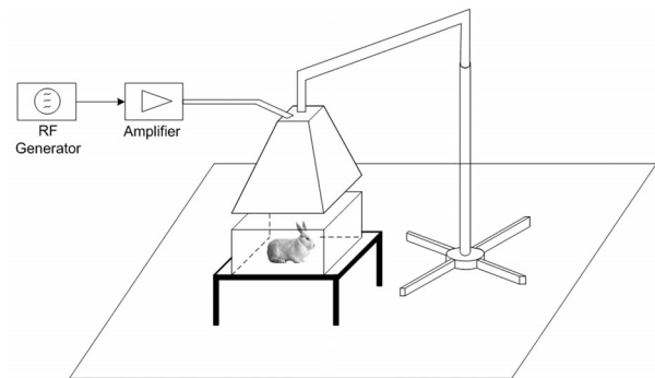
Figure 1. GSM-like Radiofrequency exposure system.
