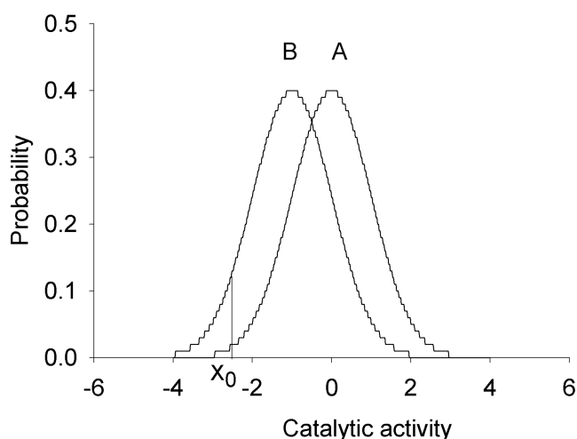
FIG. 2. Example of a genotype–phenotype association for a multifactorial phenotype. As a phenotype, standardized normal distributions of catalytic activity of a hypothetical metabolic pathway (subject to multifactorial regulation) are presented (Population A: fast metabolism; Population B: slow metabolism). X_0 reflects the threshold activity below which drug or food toxicity is observed. Note that an overlapping phenotypic distribution is a mainstay occurrence in association of a multifactorial phenotype with an omics marker. Reprinted by permission from Bentham Science Publishers: [Ozdemir et al., Curr Pharmacogenomics Person Med 2005; 3, 53–71].
