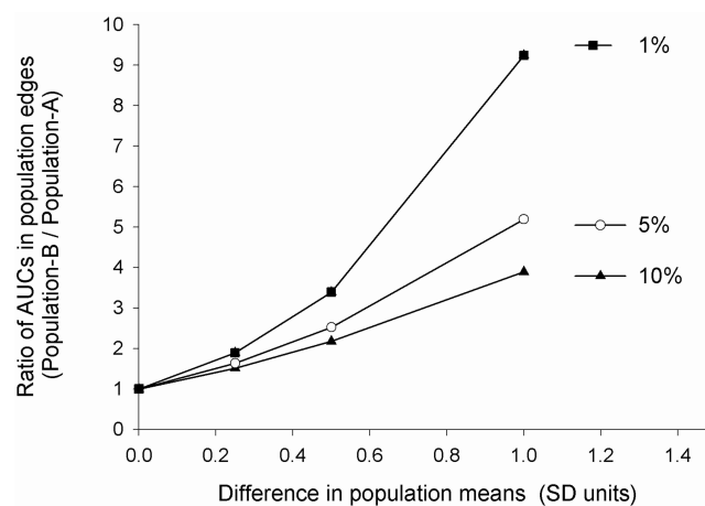
FIG. 3. Ratio of AUCs at two population edges (B/A) as a function of differences in population means when the toxicity threshold is positioned at the 10th, 5th, or the 1st percentile in the reference population A. Note the upward concavity and the nonlinear increase in the ratio of edge AUCs (population B/population A) ( ordinate ) with linear increments in the difference between population means ( abscissa ).
