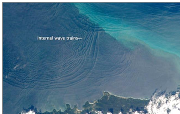
Figure 8: Image taken from the International Space Station shows Internal Waves moving through the Caribbean. Image by NASA (2013).
