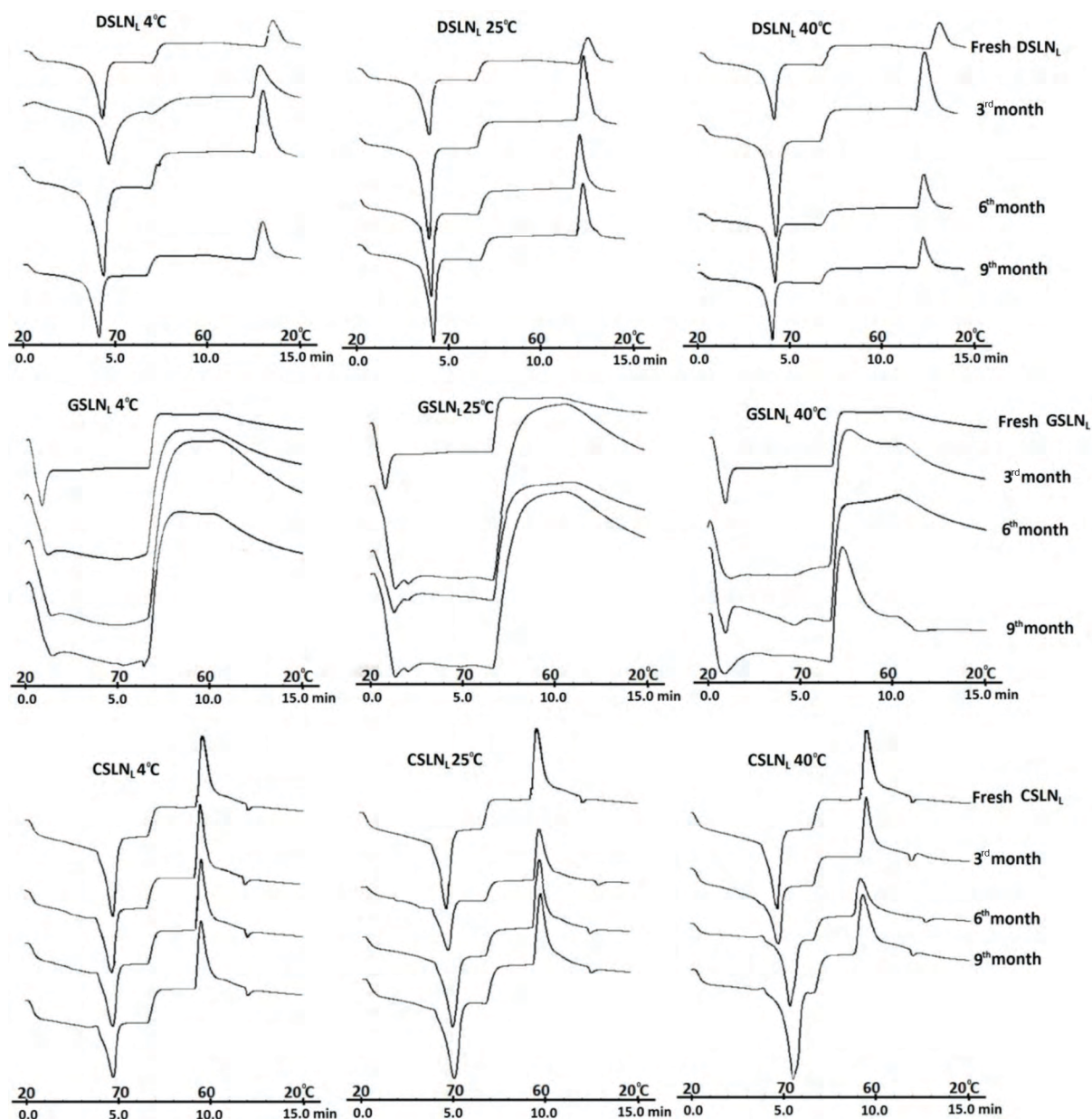
Figure 3. DSC curves of lyophilized SLNs stored at different conditions.
