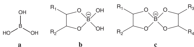
Fig. 1 (a) Boric acid, (b) anionic monoesters and (c) anionic diesters with organic molecules bearing cis -hydroxy groups (R=H, alkyl, aryl, acyl).
