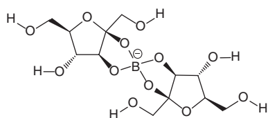
Fig. 2 Chemical structure of the fructo-borate complex anion.
