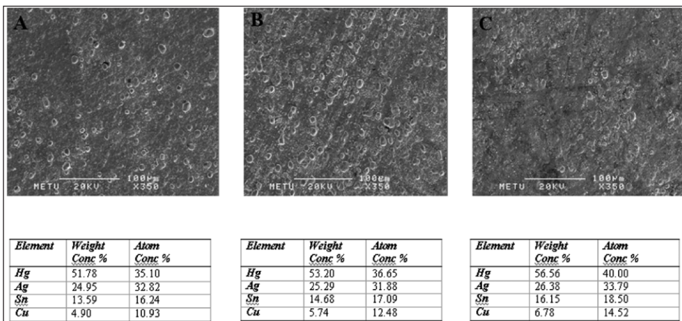
Figure 4: Scanning electron photograph (350x) and surface levels of Hg, Ag, Sn and Cu of Permite C. A: before treatment; B: after treatment with 16% CP; C: after treatment with 30% CP.
