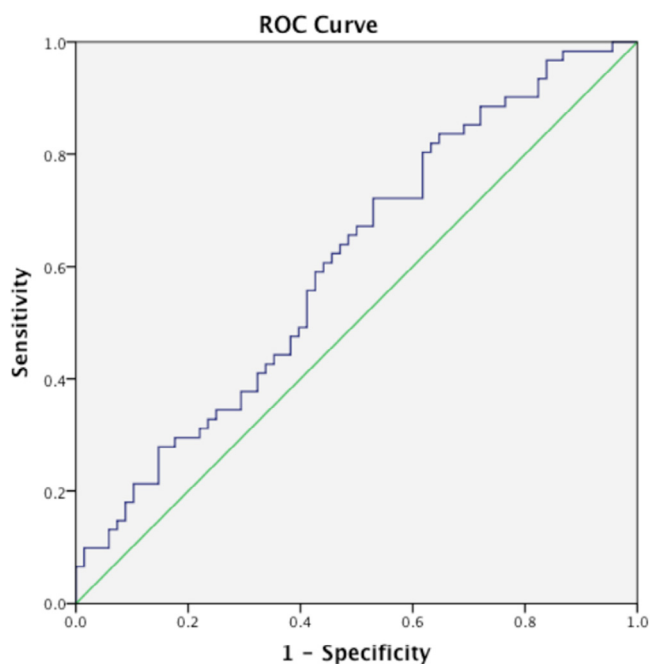
Figure 1 – Receiver operator characteristics curve of duration of blastulation (tB–tSB) to predict ongoing pregnancy. Area under curve (95% CI 0.61; 0.51 to 0.70). ROC, receiver operator characteristic.
