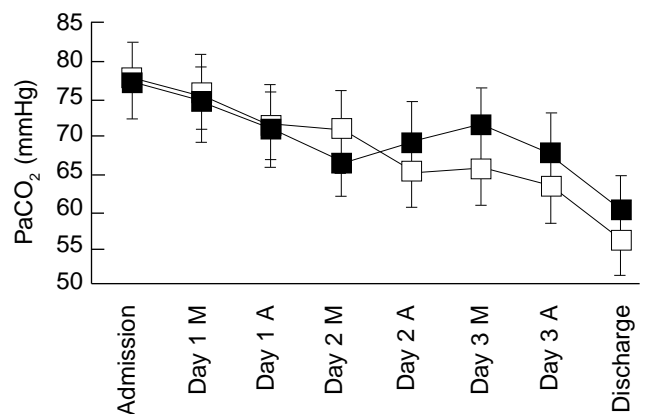
Figure 2. Changes in arterial carbon dioxide pressure ( PaCO_2 ) from admission to discharge in the active cycle of breathing techniques (ACBT) and control groups. \square = ACBT group, \blacksquare = control group, M = morning, A = afternoon. Data are means and standard deviations.
