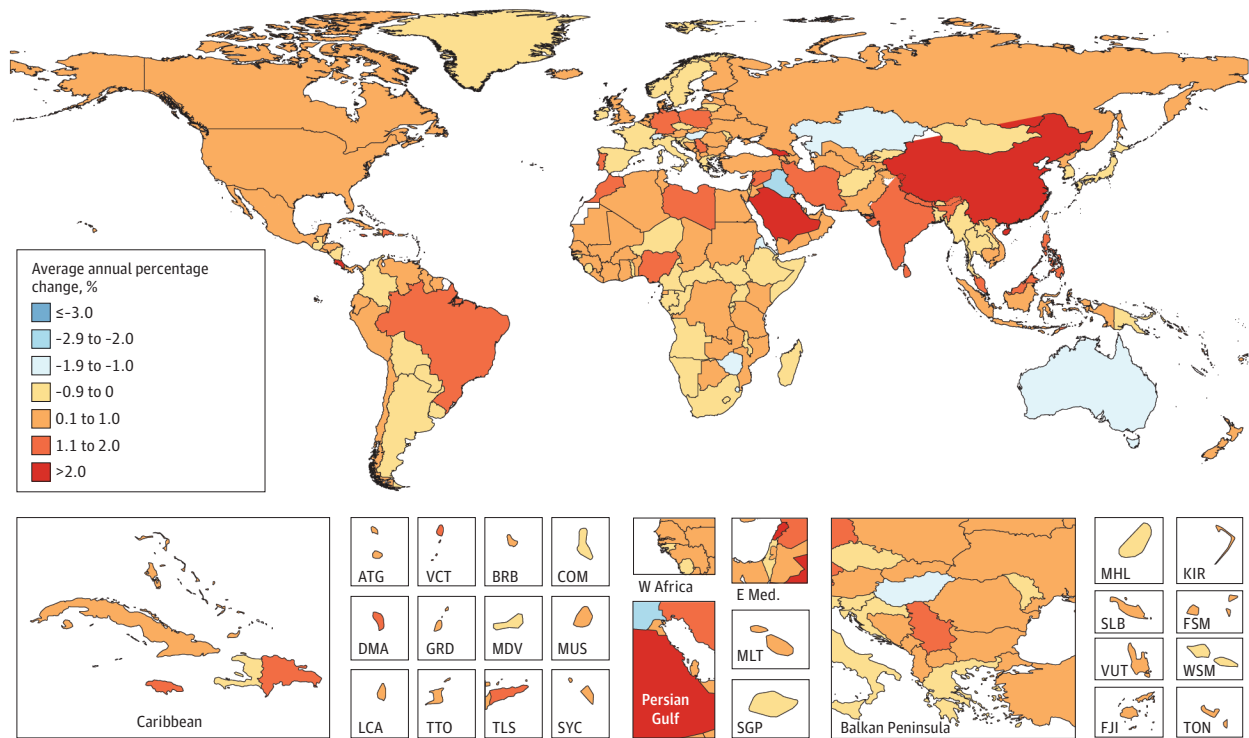
Figure 1. Average Annual Percentage Change in Age-Standardized Incidence Rate in Both Sexes for All Cancers From 2007 to 2017
