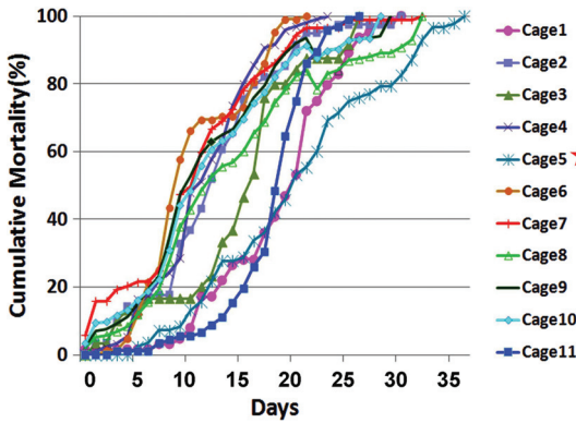
Fig. 3. Average cumulative mortality of bees kept in different cages. The bees in Cage-5 (highlighted by a star) displayed the longest survival curve among all examined cages. To improve visualization, the error bars at each time point are not shown in the figure.
