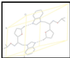
Fig. 2. A partial packing diagram of the title compound. Hydrogen bonds are shown as dashed lines. H atoms not involved in hydrogen bonding have been omitted for clarity.
