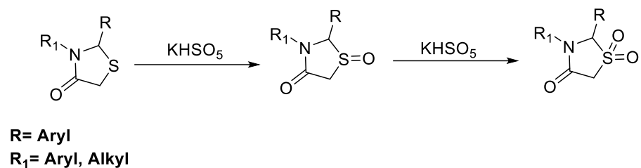
Figure 2.34. Reaction of 2,3-disubstituted-4-thiazolidinone derivatives with potassium peroxymonosulfate.
