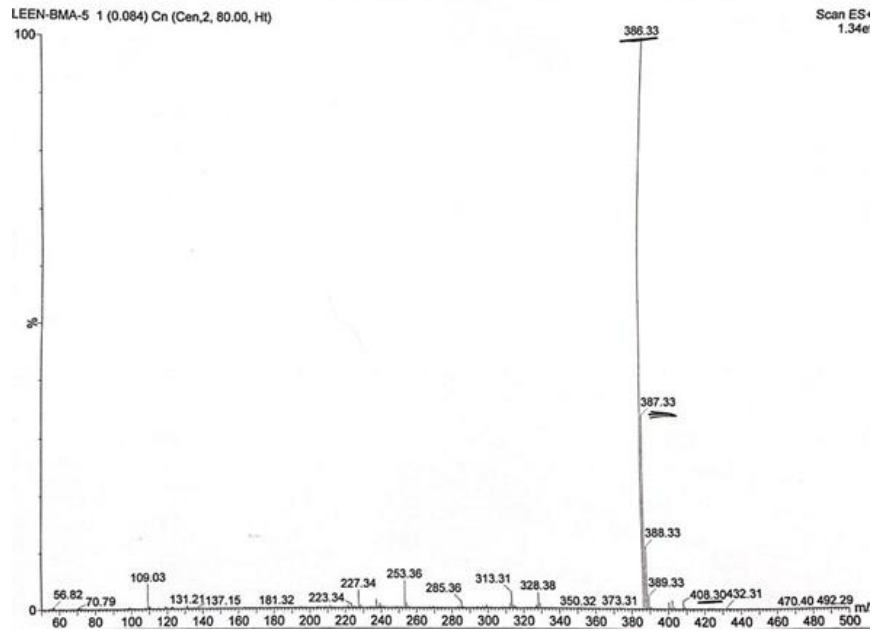
2-(4-(1 H -benzimidazol-1-yl)phenyl)-3-(3-methoxyphenyl)thiazolidin-4-one
