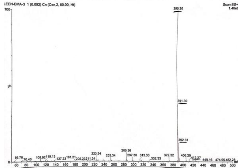
2-(4-(1 H -benzimidazol-1-yl)phenyl)-3-(4-methylphenyl)thiazolidin-4-one
