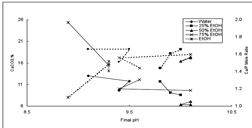
Figure 5. Effect of solvent on the reaction at 80°C.
