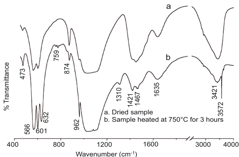
Figure 8. FT-IR spectra of the dried and the heated samples.
