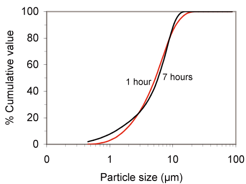
Figure 6. Effect of reaction time on the particle size of the products.
