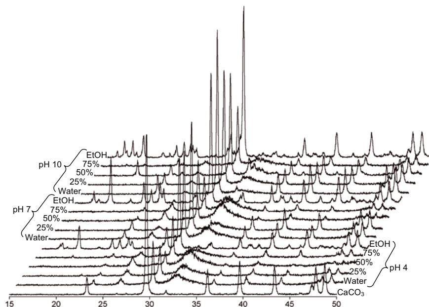
Figure 2. XRD patterns of the products obtained at room temperature.
