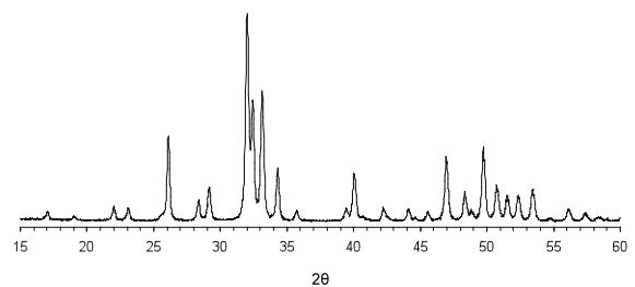
Figure 7. XRD pattern of the product heated at 750°C.
