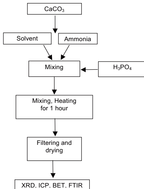
Figure 1. Flow sheet of the experiments.
