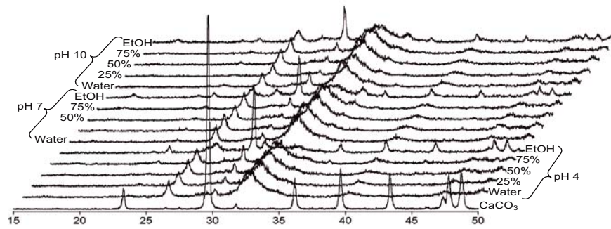
Figure 4. XRD patterns of the products obtained at 80°C.
