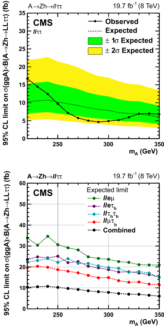
Fig. 10. Upper limits at 95% CL on cross section times branching fraction on A \rightarrow \text{Zh} \rightarrow \text{LL}\tau\tau for all ll\tau\tau final states combined (top) and comparison of the different final states (bottom).
