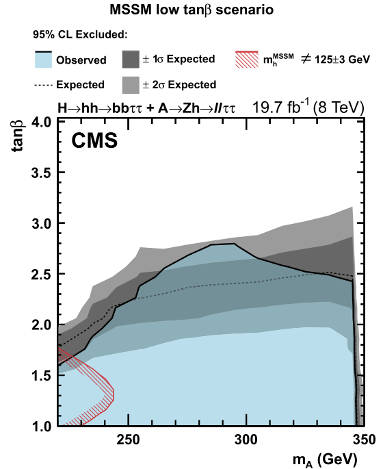
Fig. 11. The 95% CL exclusion region in the m_A - \tan\beta plane for the low \tan\beta scenario as discussed in the introduction, combining the results of the H \rightarrow \text{hh} \rightarrow \text{bb}\tau\tau and the A \rightarrow \text{Zh} \rightarrow \text{ll}\tau\tau analysis. The area highlighted in blue below the black curve marks the observed exclusion. The dashed curve and the grey bands show the expected exclusion limit with the relative uncertainty. The red area with the back-slash lines at the lower-left corner of the plot indicates the region excluded by the mass of the SM-like scalar boson being 125 GeV. The limit falls off rapidly as m_A approaches 350 GeV because decays of the A to two top quarks are becoming kinematically allowed. (For interpretation of the references to colour in this figure legend, the reader is referred to the web version of this article.)
